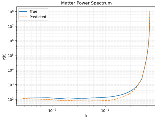
Figure 5.5: Matter Power Spectrum of UNet-VAE
