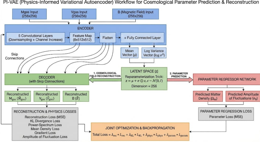
Figure 4.2: Architecture and Workflow of the Proposed PIVAE model
