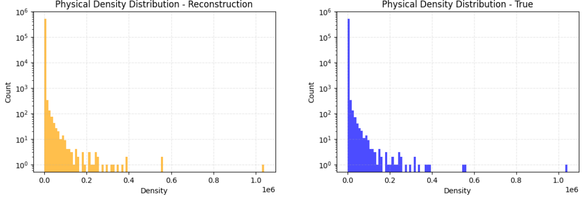
Figure 5.7: Physical Density Distribution of PI-VAE
