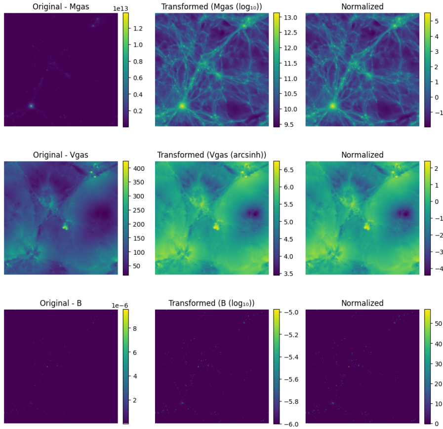
Figure 4.1: LH Set Data (before and after transformation)
