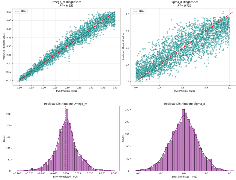
Figure 5.8: PI-VAE scatter plot and residual distribution for \Omega_m and \sigma_8
