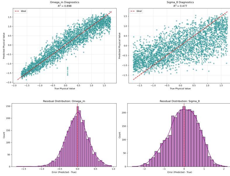
Figure 5.9: UNet-VAE scatter plot and residual distribution for \Omega_m and \sigma_8
