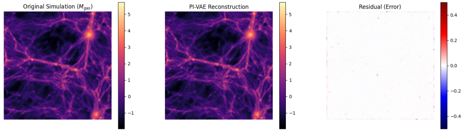
Figure 5.3: Reconstruction of Cosmological Field using PI VAE
