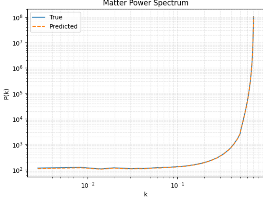
Figure 5.4: Matter Power Spectrum of PI-VAE
