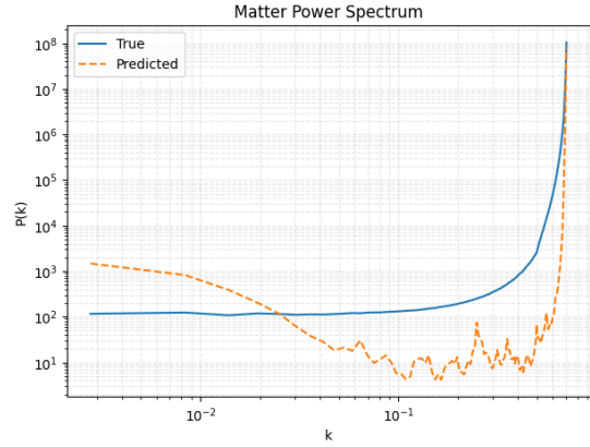
Figure 5.6: Matter Power Spectrum of VAE
