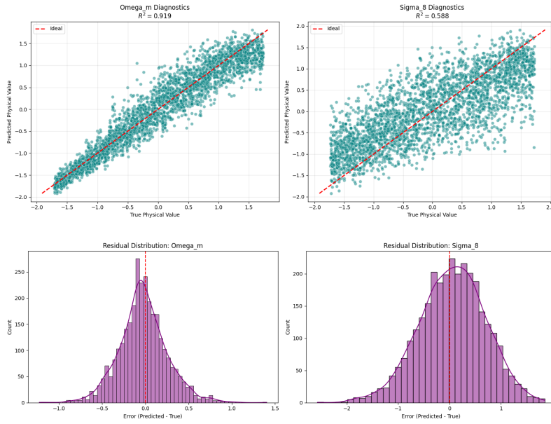
Figure 5.10: VAE scatter plot and residual distribution for \Omega_m and \sigma_8
